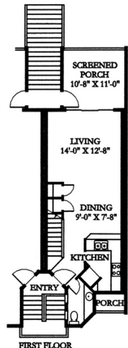
TWO BEDROOM TOWNHOUSE
