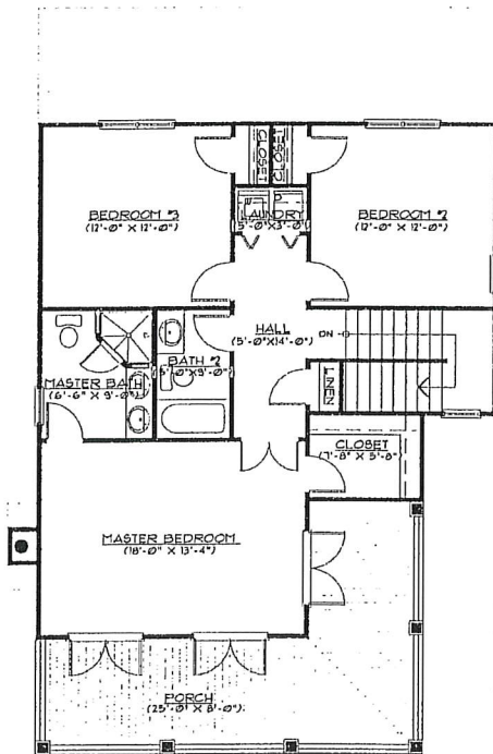
SECOND FLOOR PLAN HEATED SPACE 936 SQ. FT.
