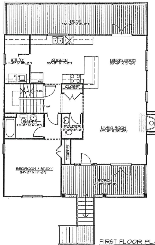
FIRST FLOOR PLAN HEATED SPACE 1,408 SQ. FT.
